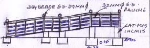
RAMP LONGITUDINAL SECTION.
