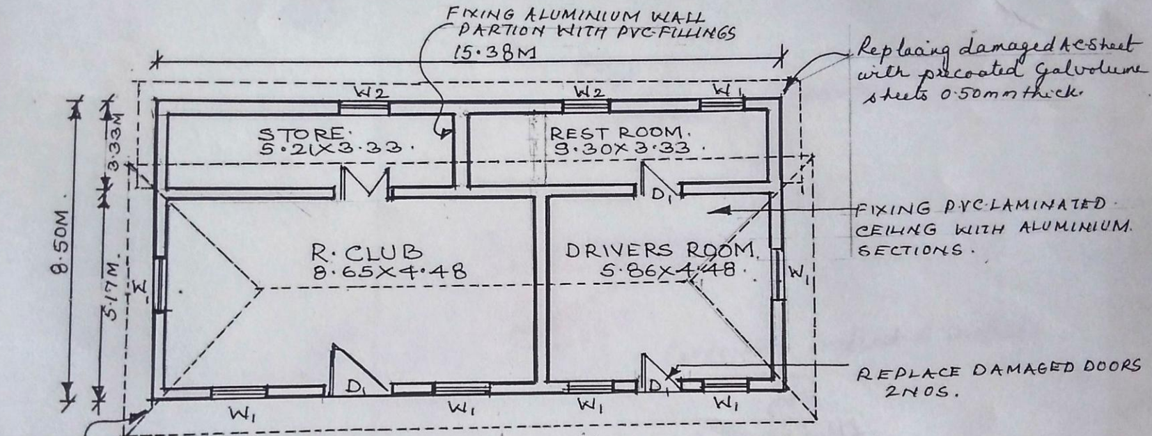
PLAN OF DRIVERS ROOM.
