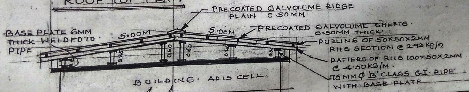
CROSS SECTION - A.B.
