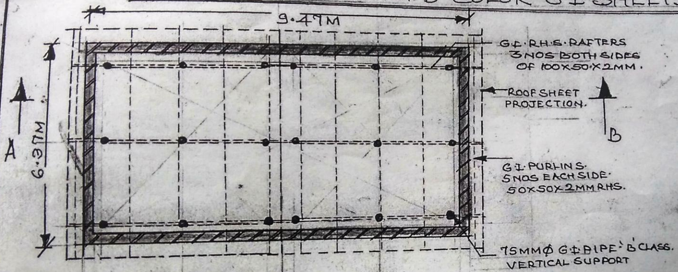
ROOF TOP PLAN.
