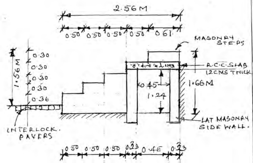
CROSS SECTION.
