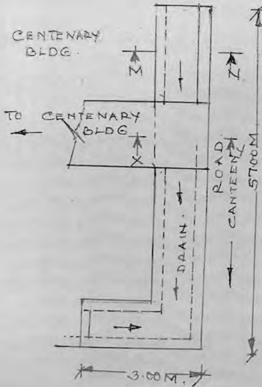
PLAN OF DRAIN.
