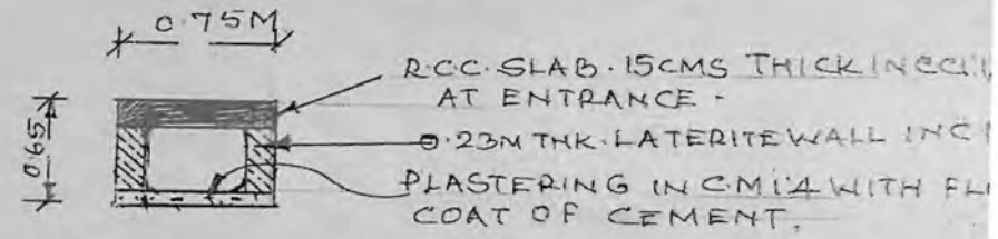
SECTION AT X-Y.
