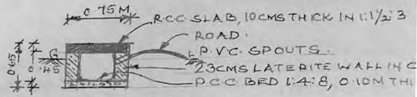
SECTION AT M-N.
