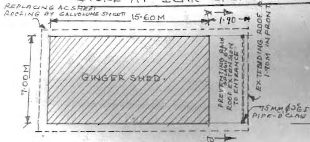
EXISTING PLAN OF GINGER SHED.
