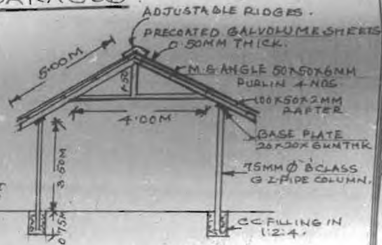
SECTION AT AB.
