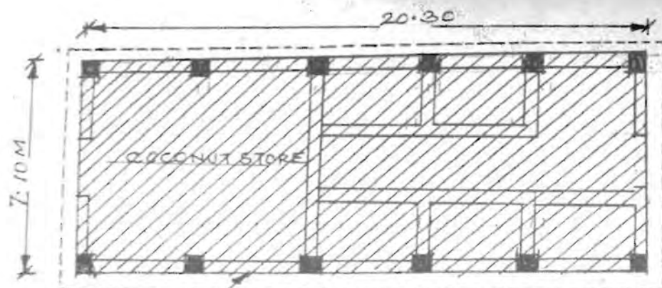
REPLACING DAMAGED WINDOW WITH CEMENT JAM. EXISTING PLAN OF COCONUT STORE
