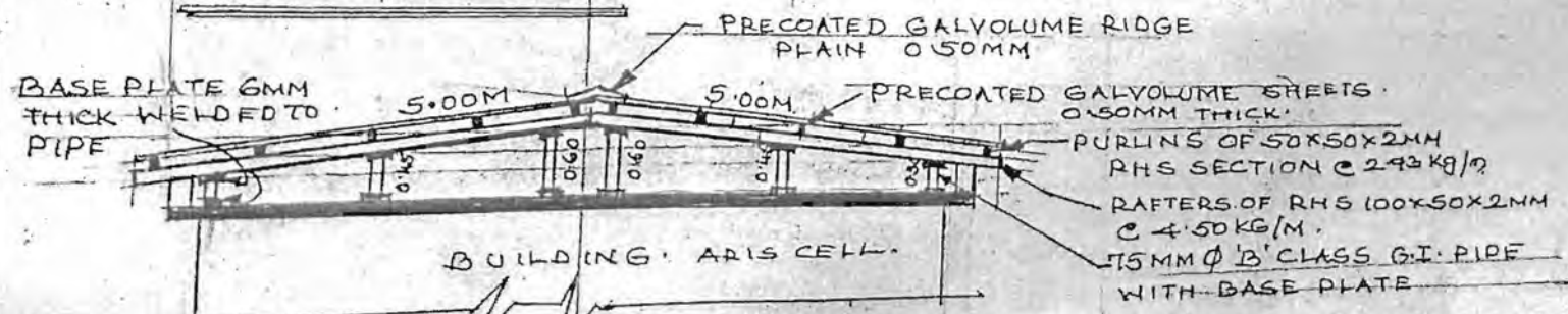
CROSS SECTION A-B
