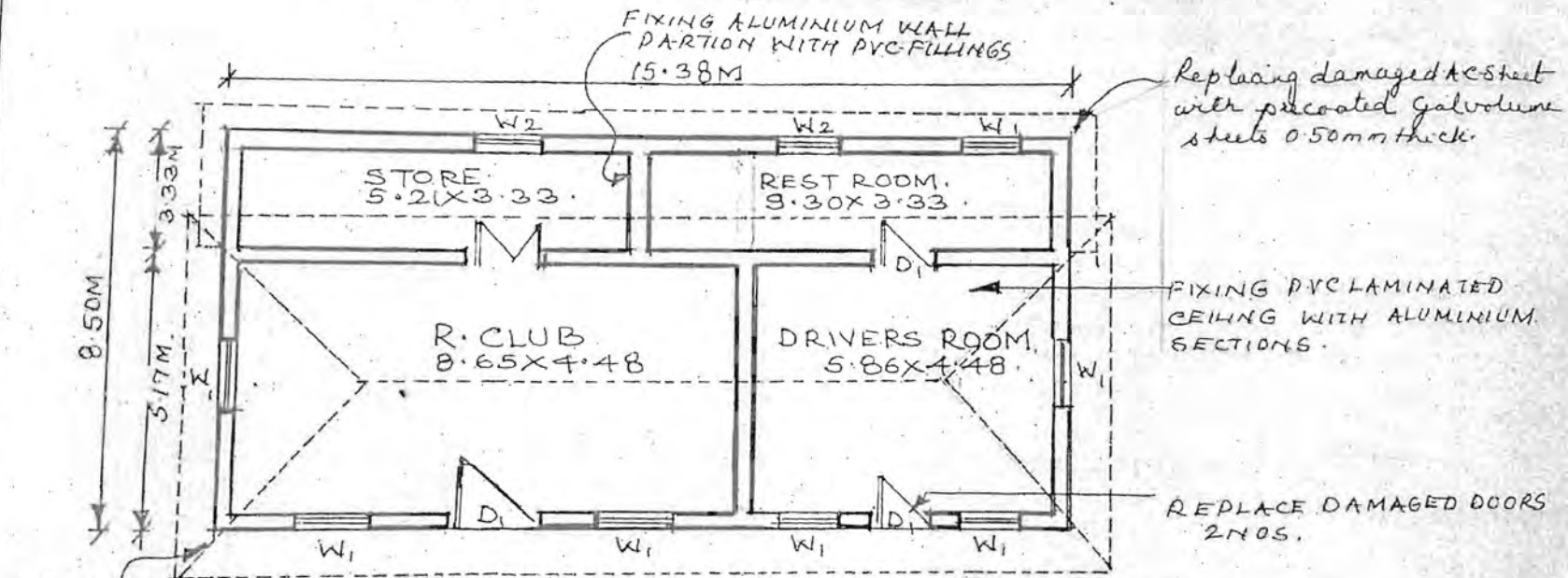
PLAN OF DRIVERS ROOM.
