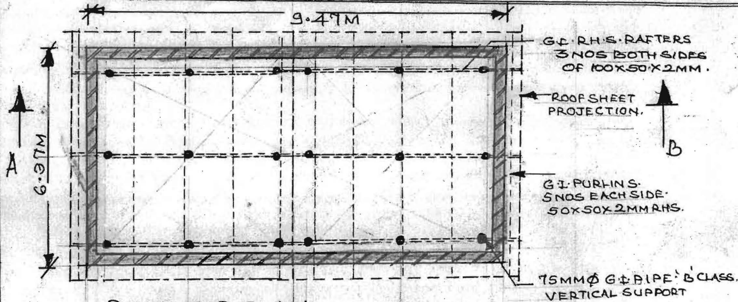
ROOF TOP PLAN.
