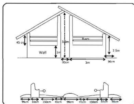
Fig.12. Elevation of the cow shed
